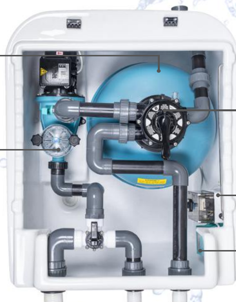
Hang-Over Filtration Units
