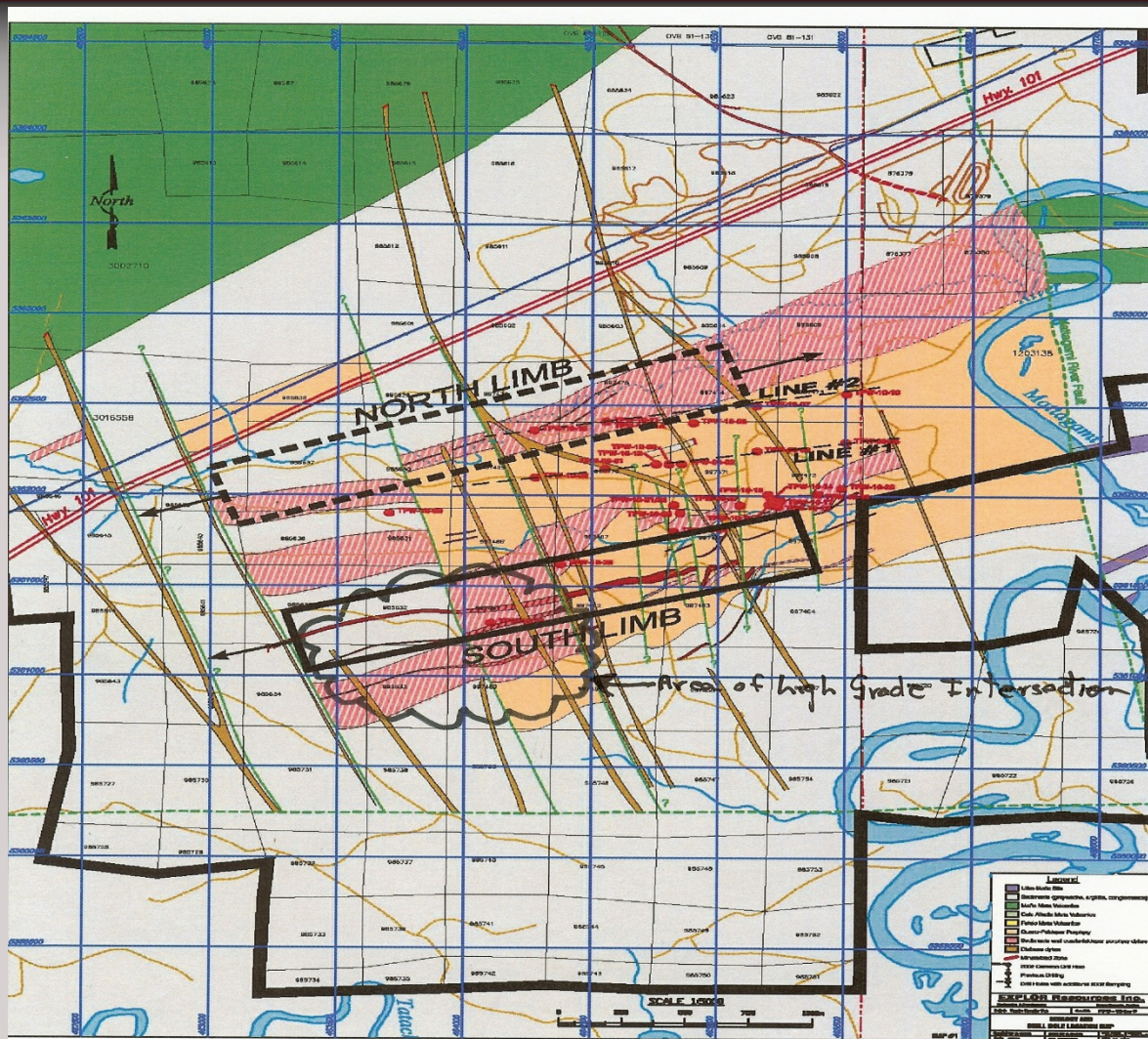
PLAN VIEW NORTH AND SOUTH LIMBS OF SYNCLINE
