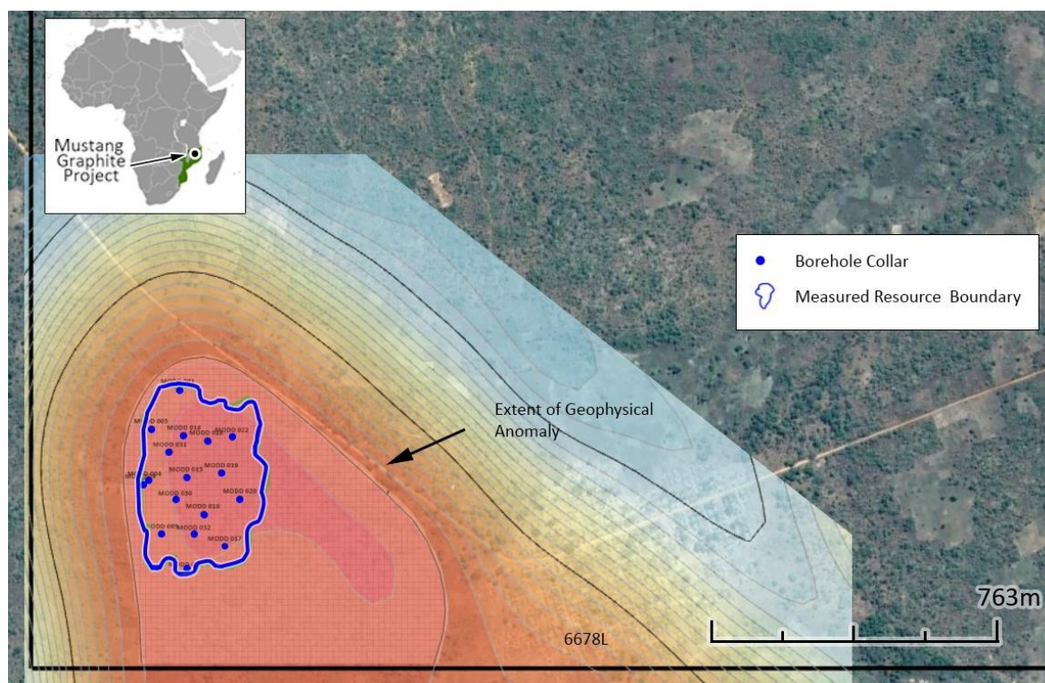
Figure 1. Locations of Drill holes and the plan view of mineralisation
