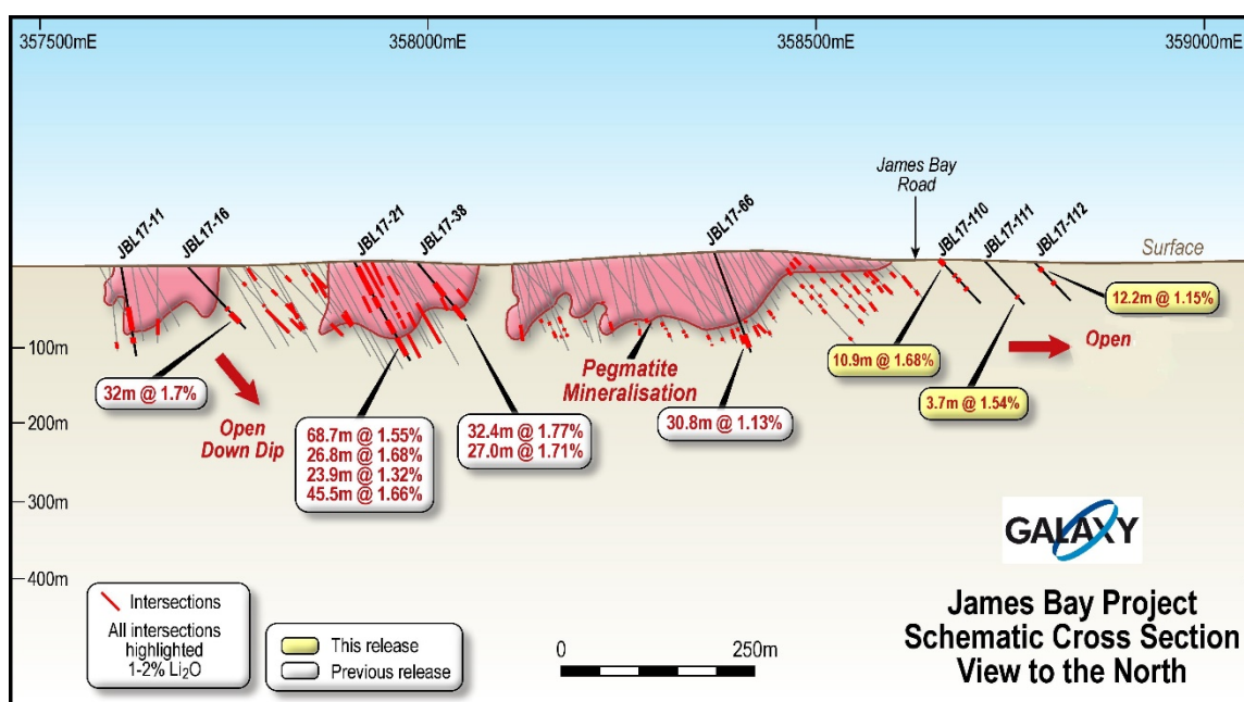
Figure 2: James Bay Spodumene Project – Section View
