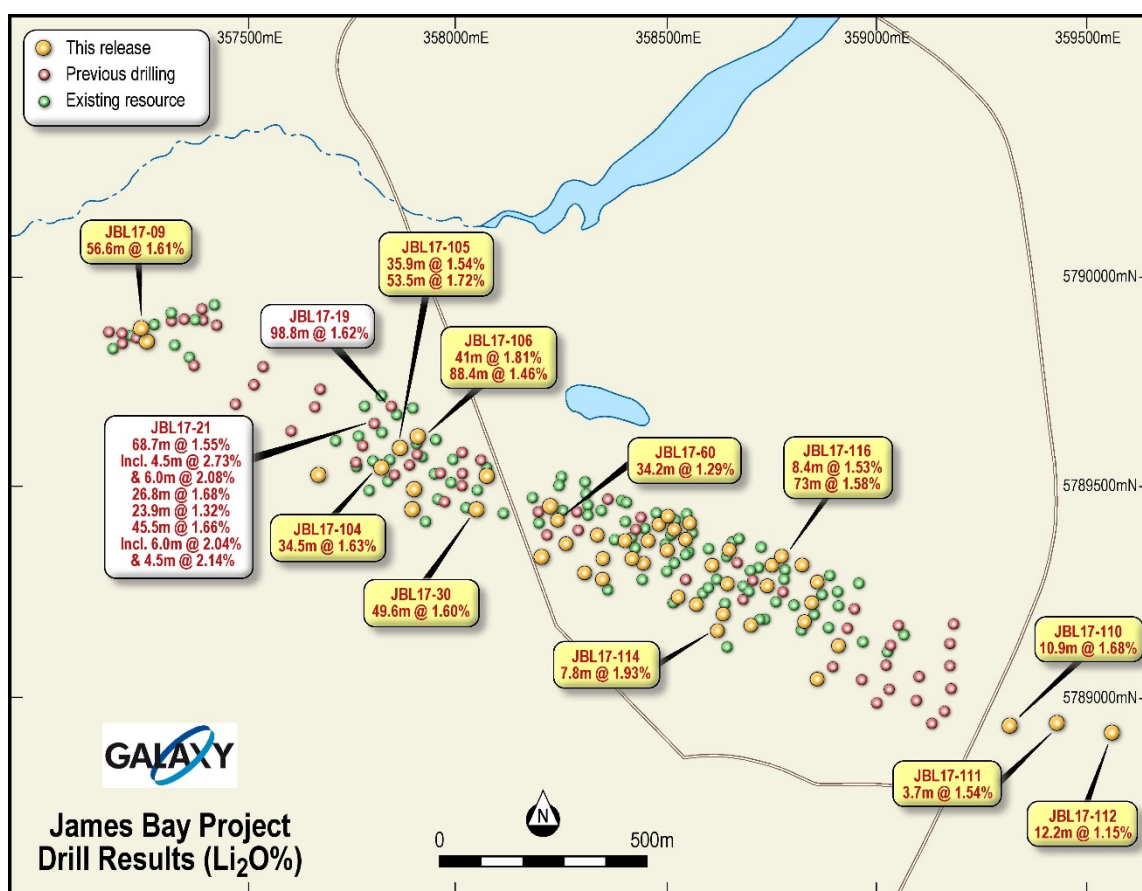
Figure 1: James Bay Spodumene Project – Plan View
