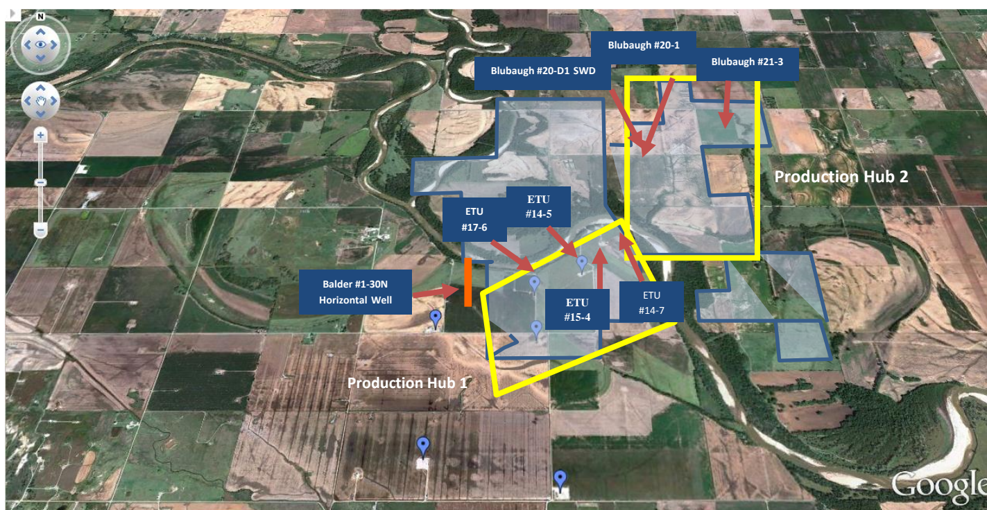
Figure 5 – Location of production hubs in southwest area of Snake River Project
