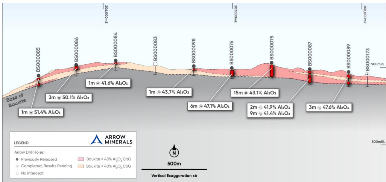
Figure 5. Boussoura Central Drill Section 1,206,700 North, analytical results reported as significant intercepts with a 40% \text{Al}_2\text{O}_3 cut-off
