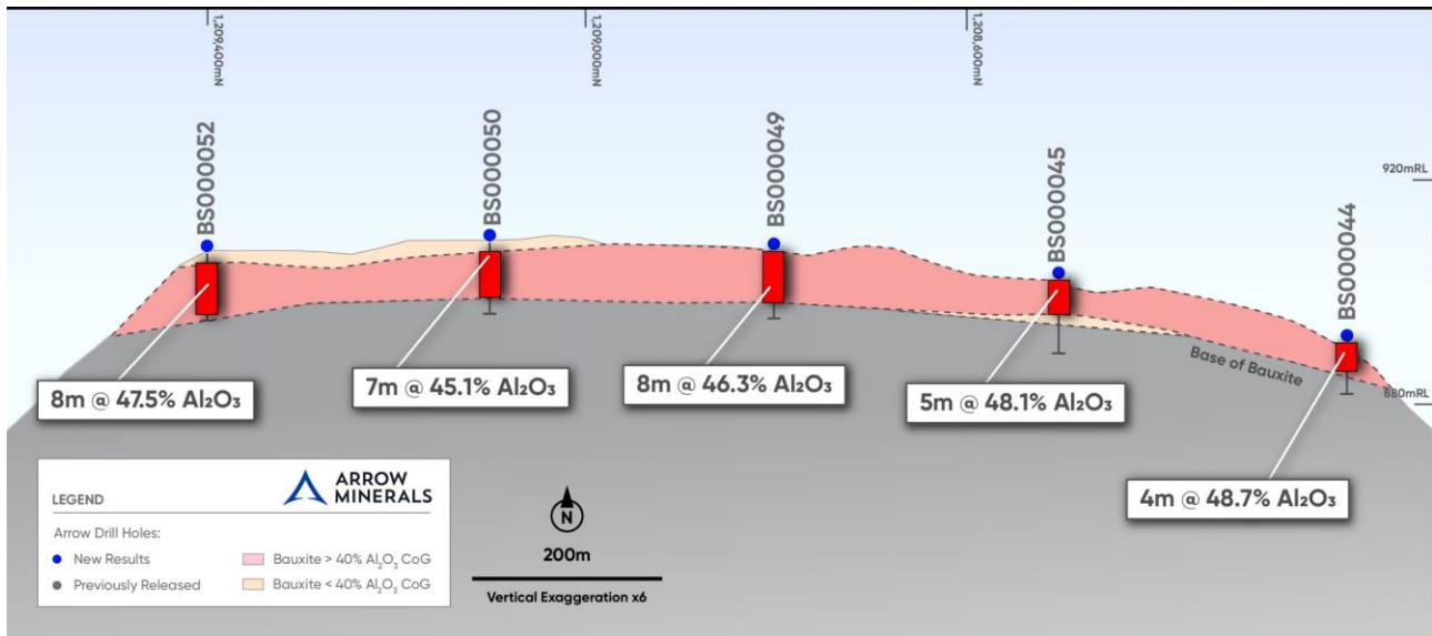
Figure 4. Boussoura North Drill Section 207,300 East, analytical results reported as significant intercepts with a 40% \text{Al}_2\text{O}_3 cut-off
