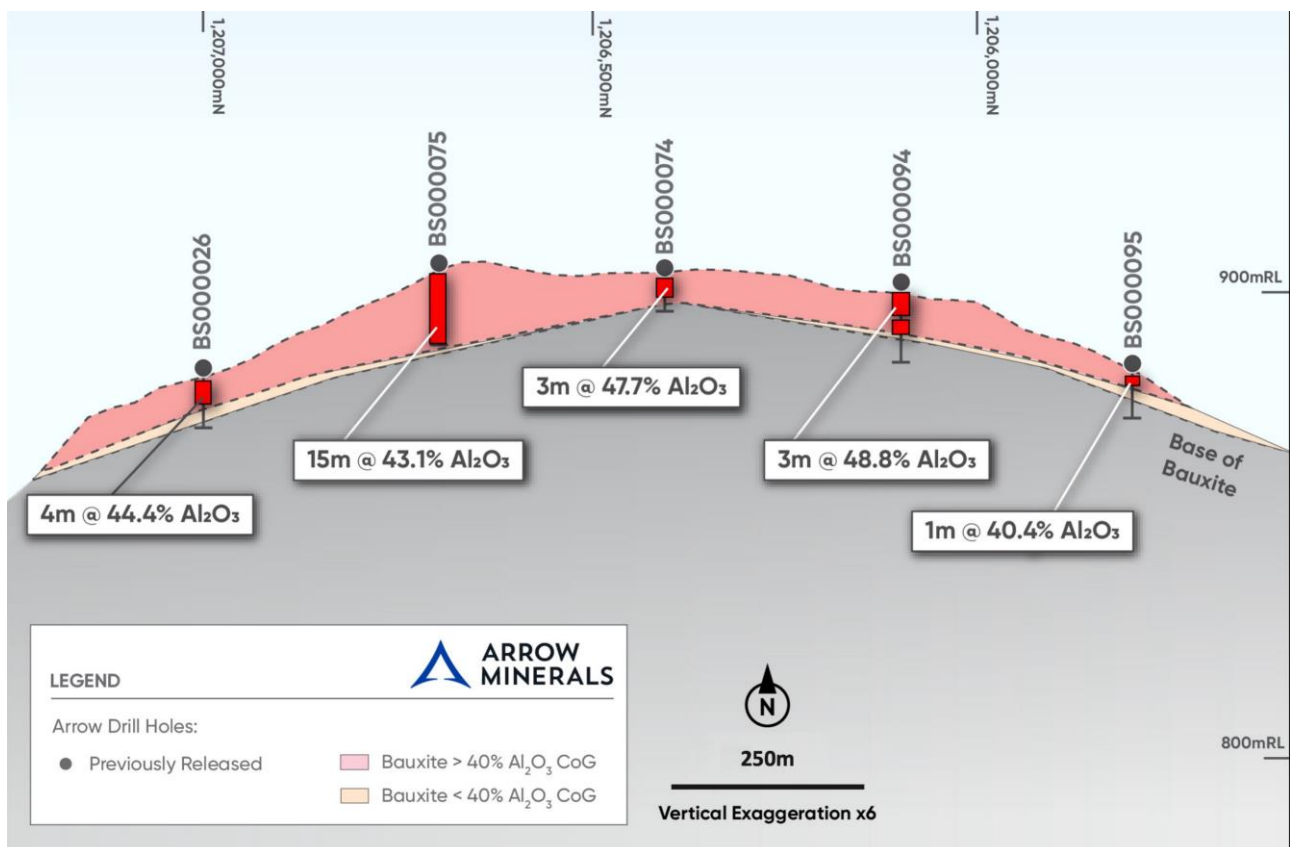
Figure 6. Boussoura Central Drill Section 207,300 East, analytical results reported as significant intercepts with a 40% \text{Al}_2\text{O}_3 cut-off
