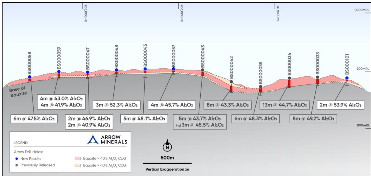
Figure 3. Boussoura North Drill Section 1,208,500 North, analytical results reported as significant intercepts with a 40% \text{Al}_2\text{O}_3 cut-off
