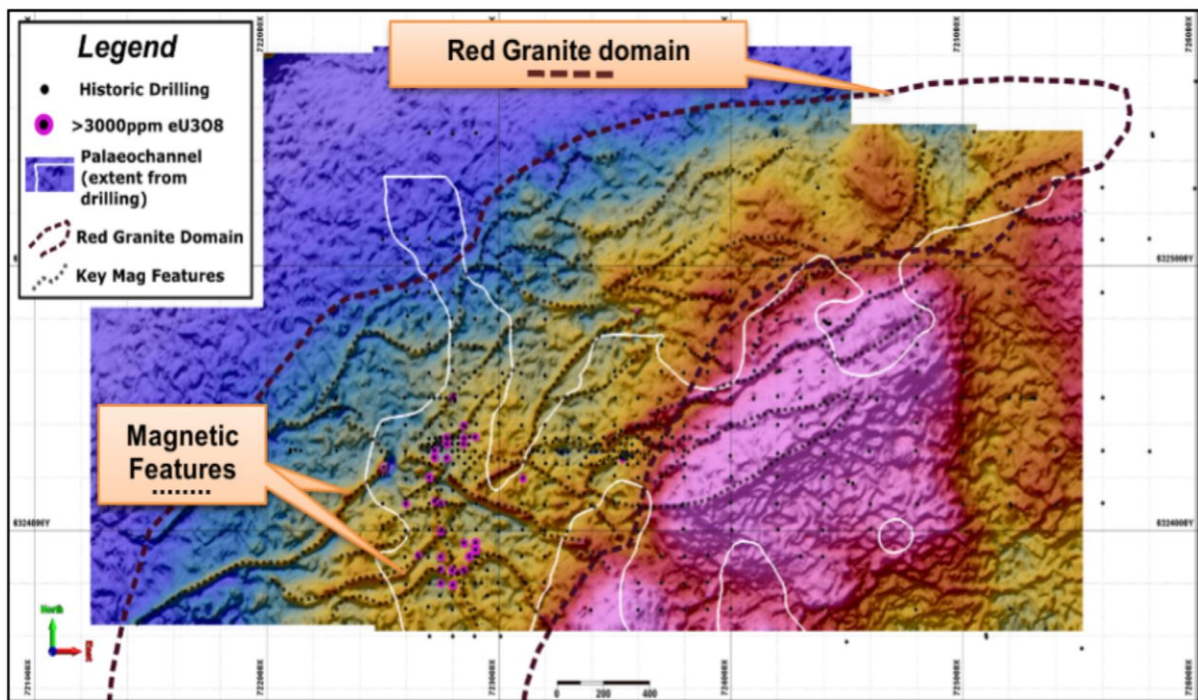
Figure 1: New high-resolution ground TMI Magnetics with hole intersects >3000ppm eU308 highlighted and northeast-southwest Mag zone.
