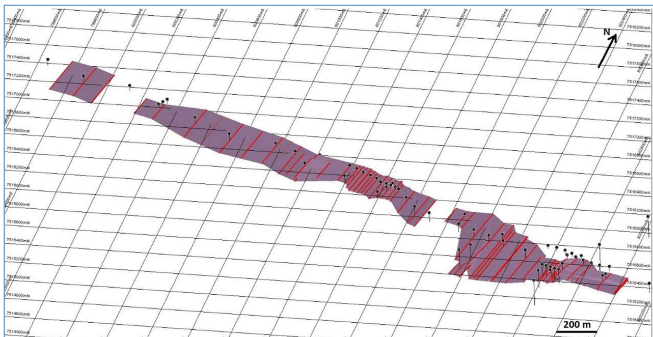
Figure 4. Wireframe models of the mineralised bodies.
