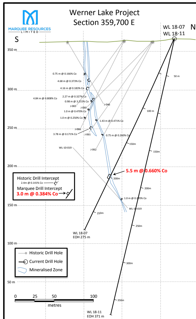
Figure 1: Simplified Cross Section 359,700 E.
