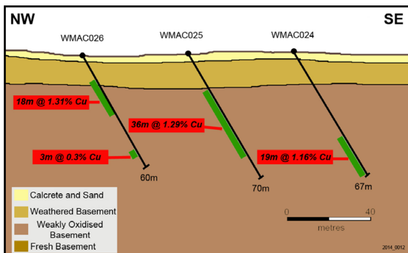
Figure 2: Champion prospect Section 2 looking northeast. High grade subzones of copper intercepted highlighted by green zones. Remaining zones contain copper < 0.1 %.
