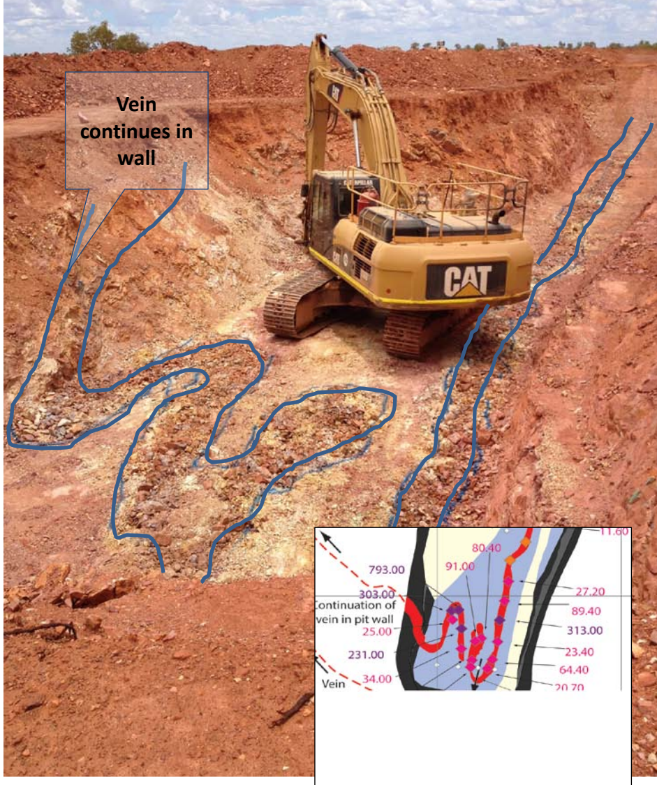
Old Pirate South – South plunging fold with high-grade gold.
