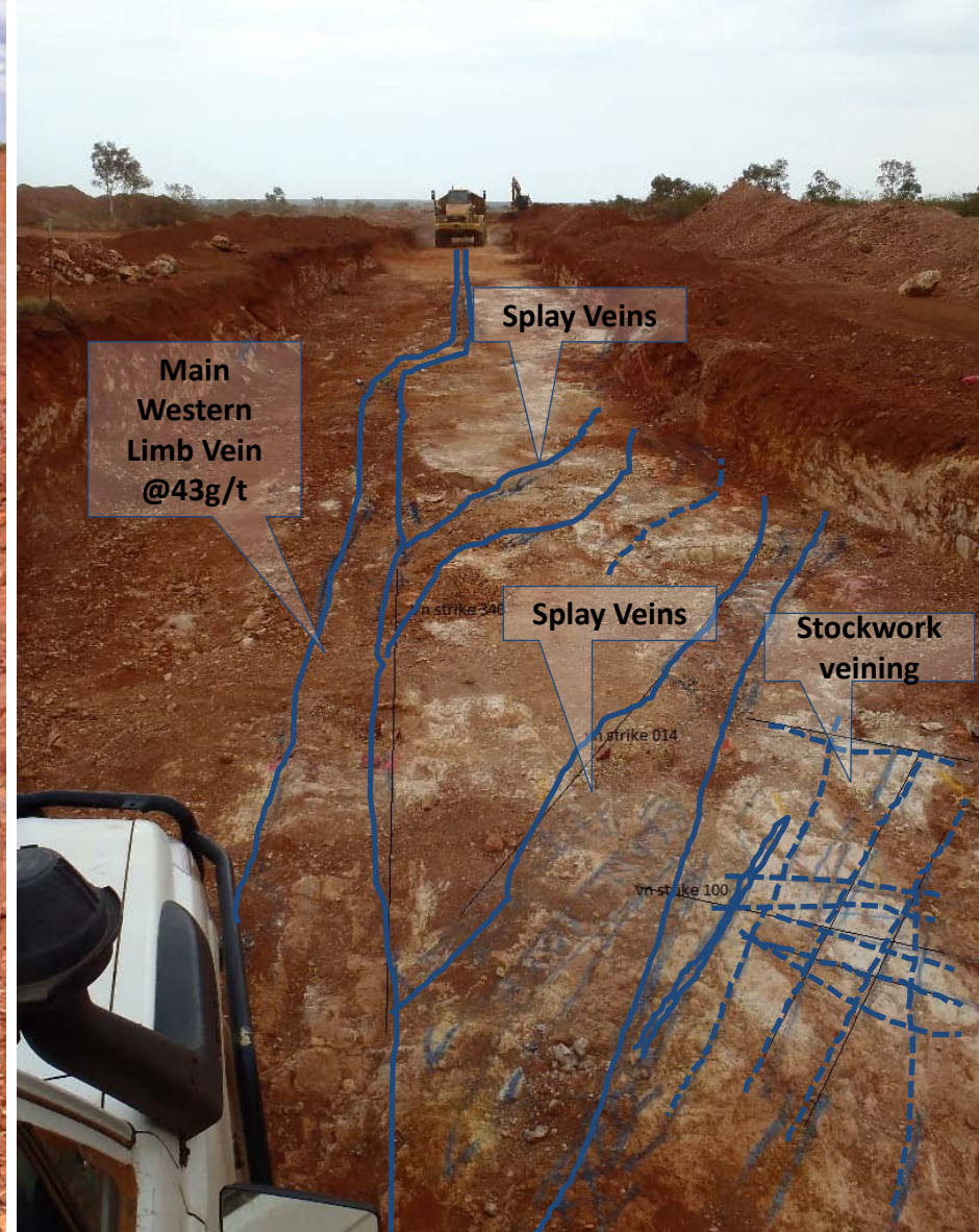
New Splay structures revealed at the Western Limb.
