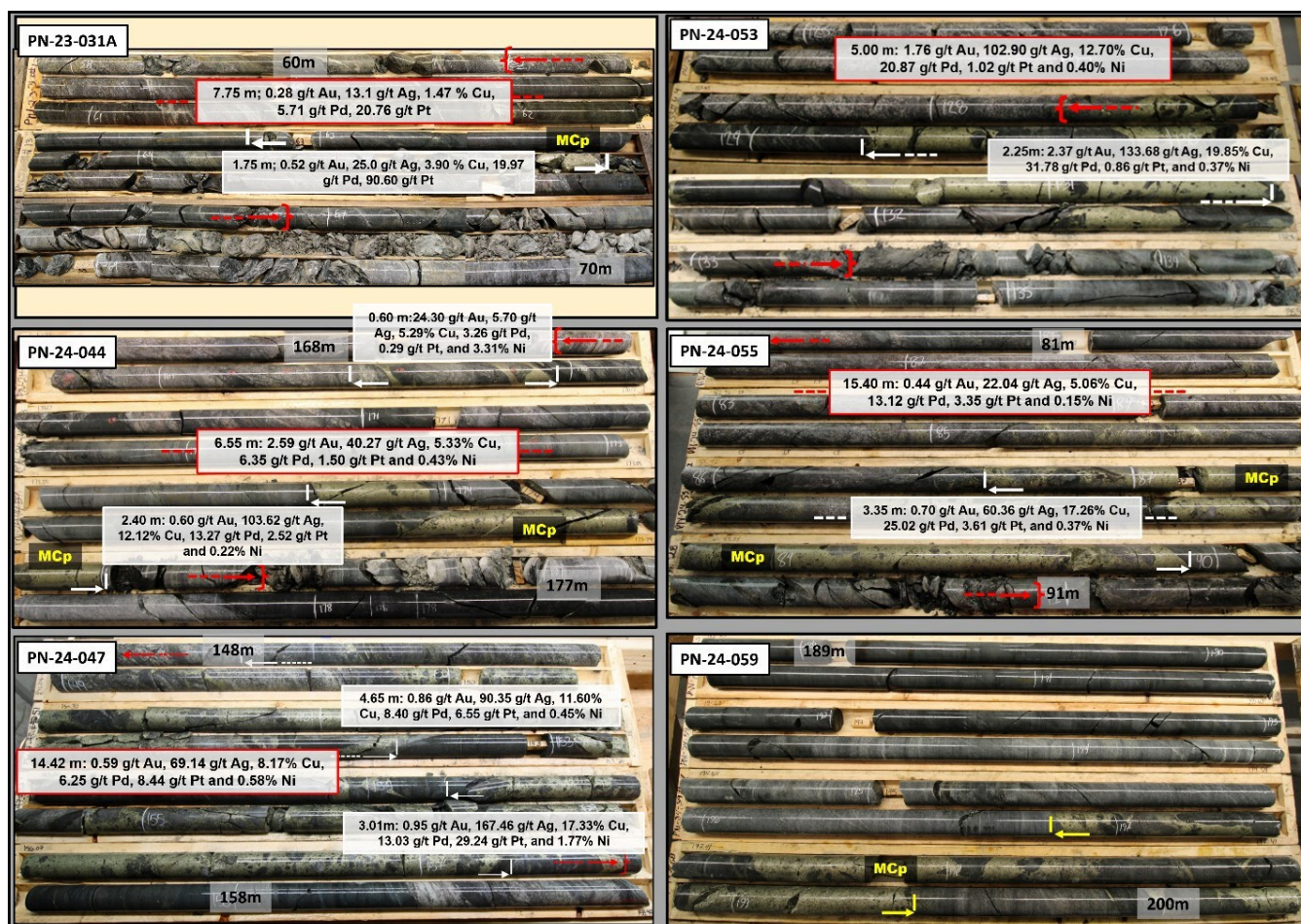
Figure 1: Core pictures showing the relation between observed massive chalcopyrite and grade, and the relative visual amount of massive chalcopyrite (MCp) observed in some of the best intersections to date.
