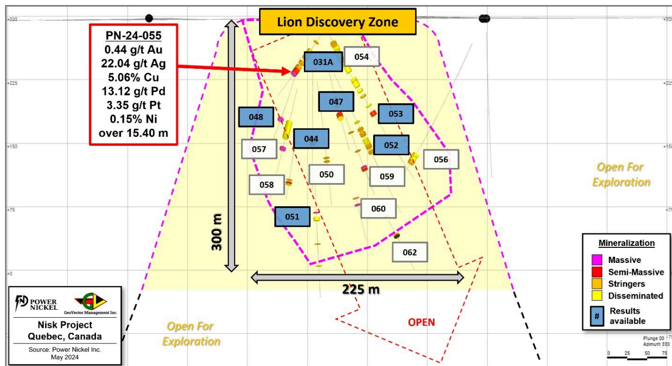
Figure 2: Longitudinal view of the Lion Discovery zone; Presenting the location of hole PN-24-055, as well as the pierce points locations of the other winter 2024 drillholes.
