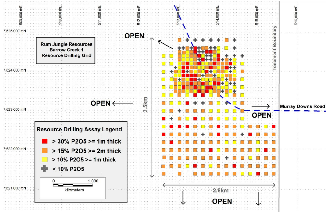
Figure 1: Distribution of Phosphate Grade over Barrow Creek 1 Resource Drilling Grid.
