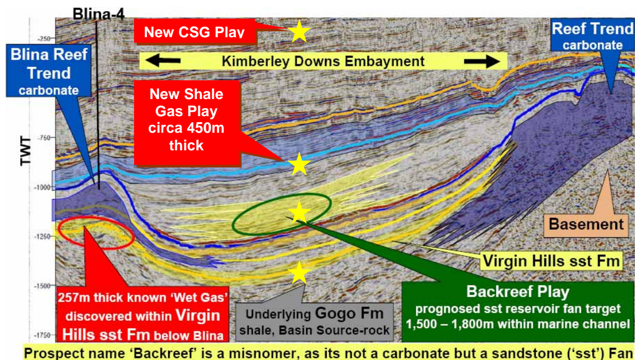
Figure 3 Backreef Prospect (drill-ready) (schematic only showing shallow CSG and deeper USG & Stratigraphic Plays)
