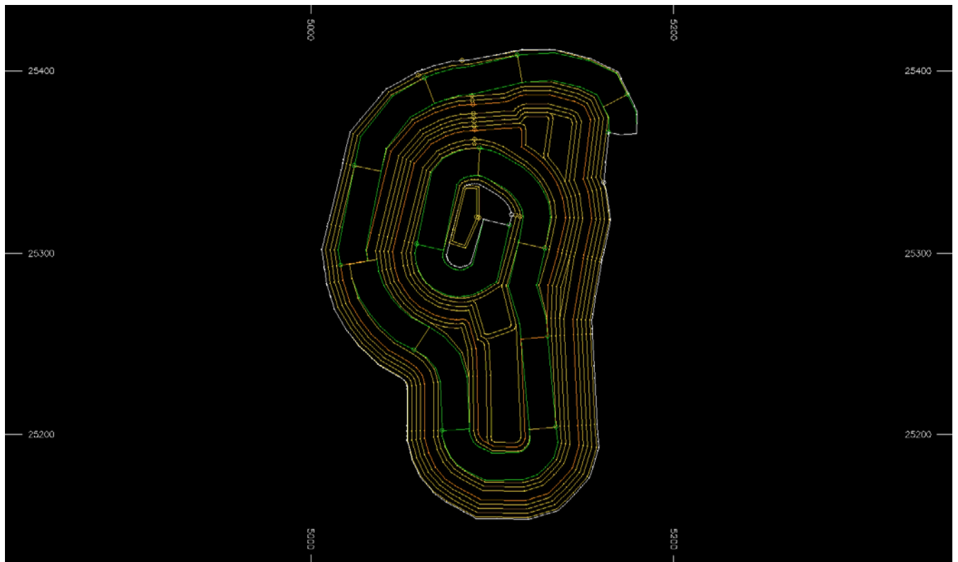
Fig 2. Coogee Deposit: Open Pit Mine Design
