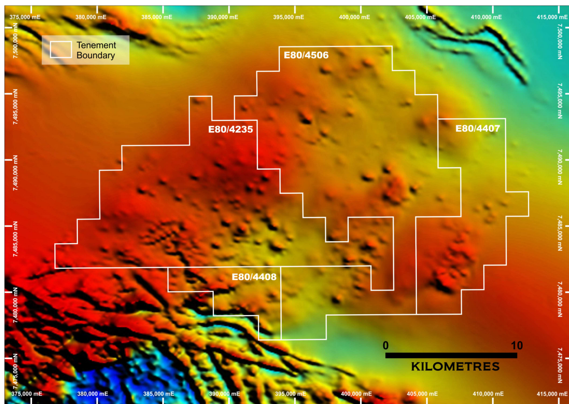
Figure 2 Aeromagnetic Image Showing Target Anomalies
