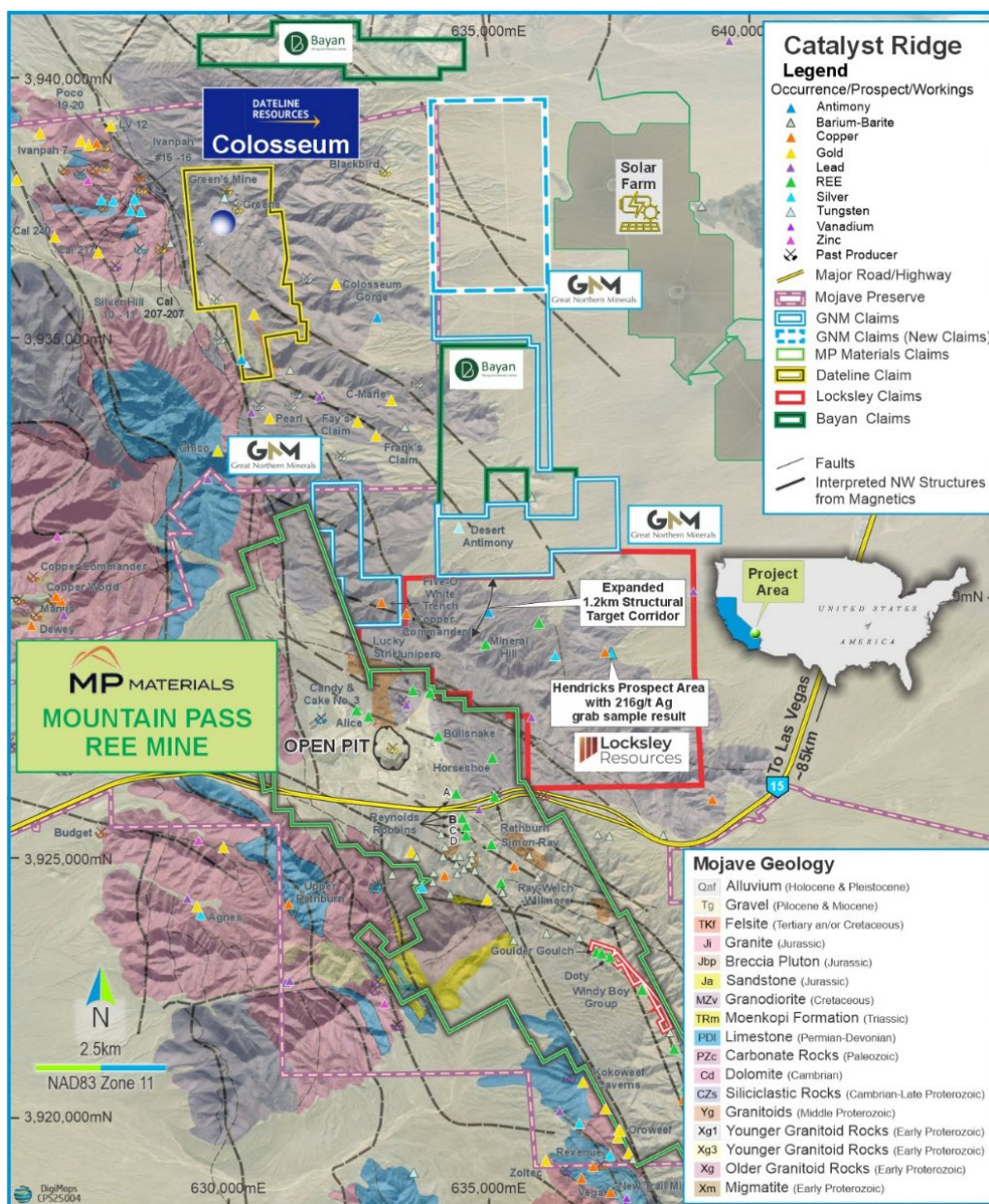
Figure 1: Interpreted bedrock geology map from the US Geological Survey 1 showing the location of the GNM claims in relation to the Mountain Pass REE deposit, associated nearby mineral occurrences and other companies in the area.
